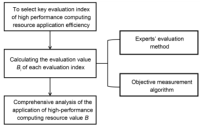
Figure 1: Evaluation process.
